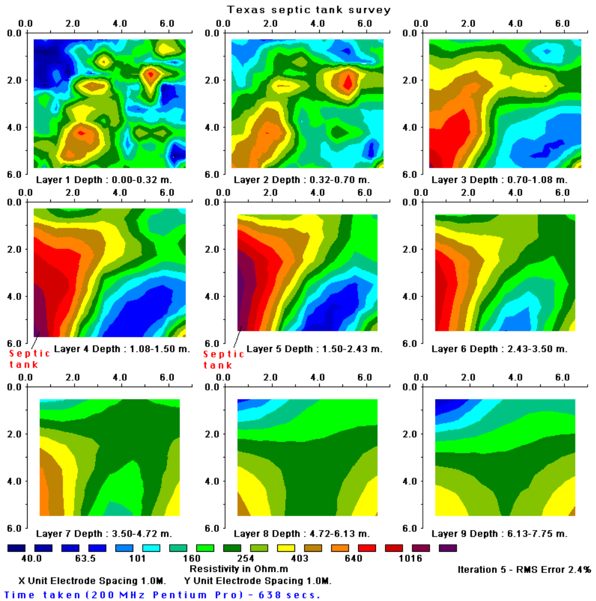
Figure 34. The model obtained from the inversion of the septic tank field survey data set. The model is shown in the form of horizontal slices through the earth.
