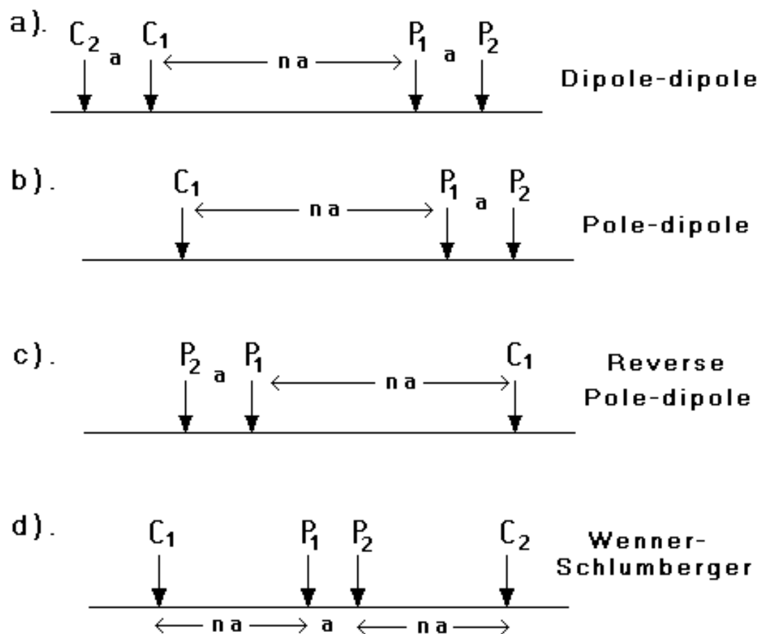
Figure 36. Arrangement of the electrodes for the dipole-dipole, pole-dipole and Wenner-Schlumberger arrays, together with the definition of the "a" spacing and the "n" factor for each array.
