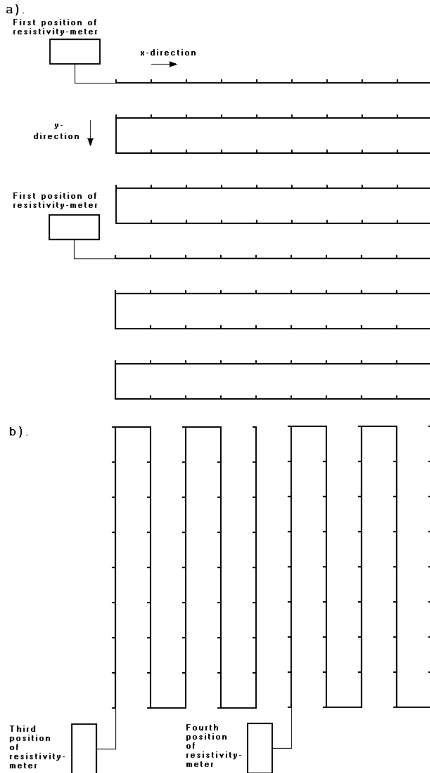
Figure 29. Using the roll-along method to survey a 10 by 10 grid with a resistivity-meter system with 50 electrodes. (a) Surveys using a 10 by 5 grid with the lines orientated in the x-direction. (b) Surveys with the lines orientated in the y-direction.
