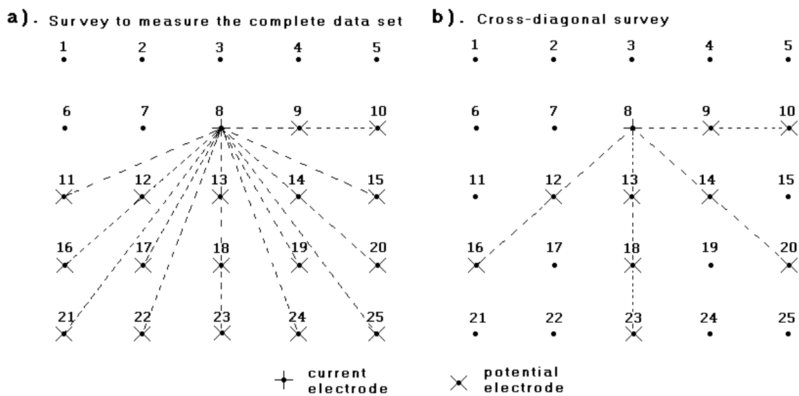
Figure 28. The location of potential electrodes corresponding to a single current electrode in the arrangement used by (a) a survey to measure the complete data set and (b) a cross-diagonal survey.
