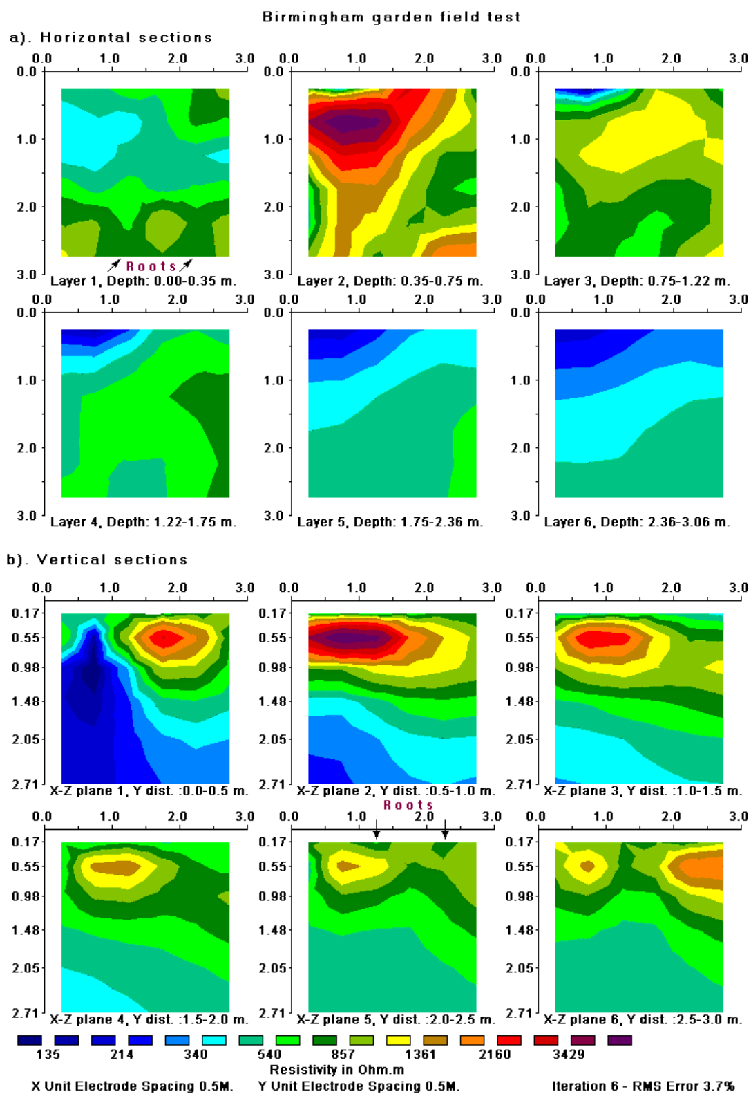
Figure 33. Horizontal and vertical cross-sections of the model obtained from the inversion of the Birmingham field survey data set. The location of observed tree roots on the ground surface are also shown.
