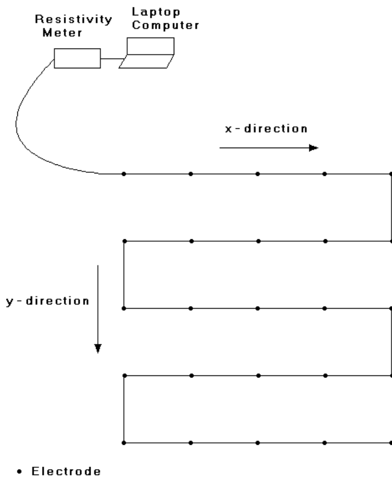
Figure 27. The arrangement of the electrodes for a 3-D survey.
