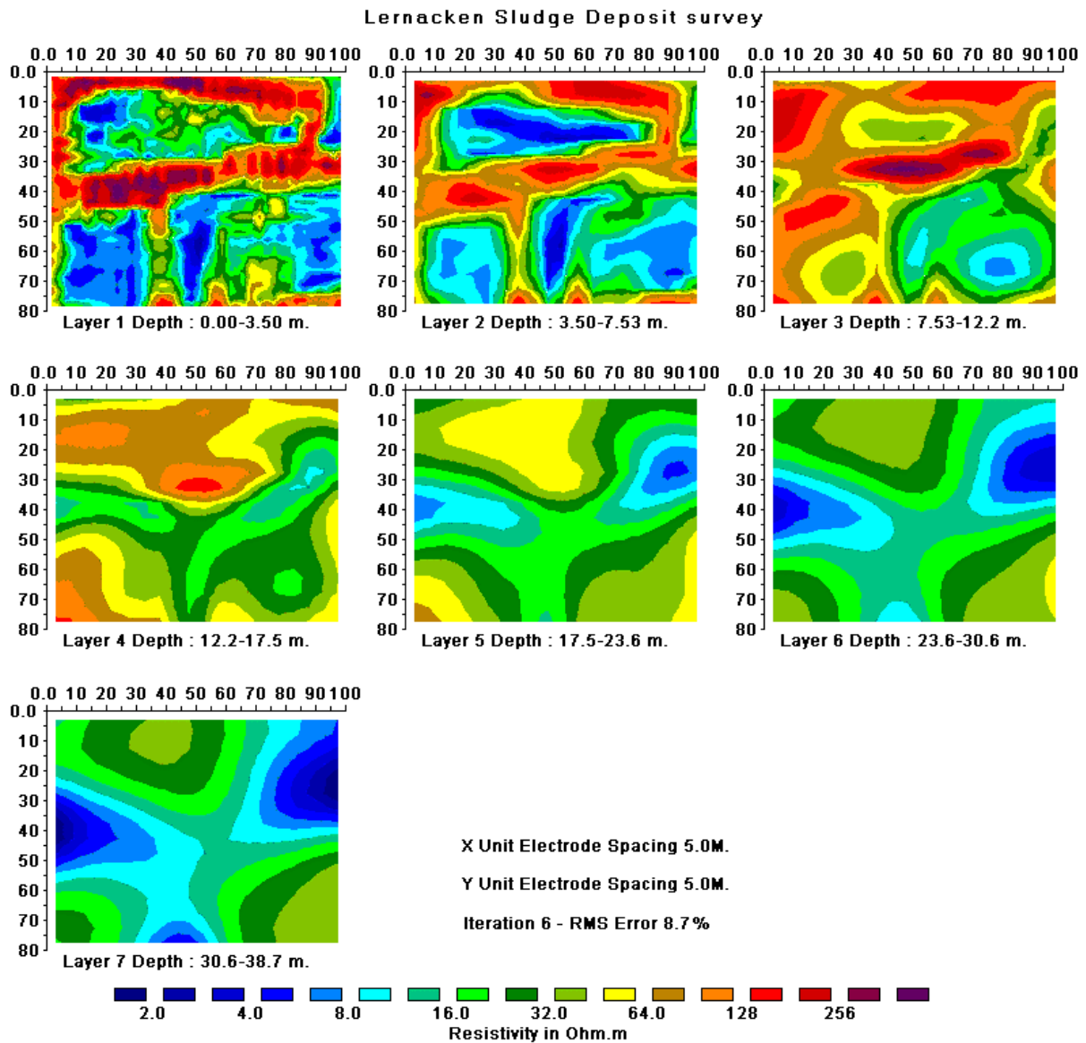
Figure 35. The 3-D model obtained from the inversion of the Lernacken Sludge deposit survey data set. The model is shown in the form of horizontal slices through the earth.
